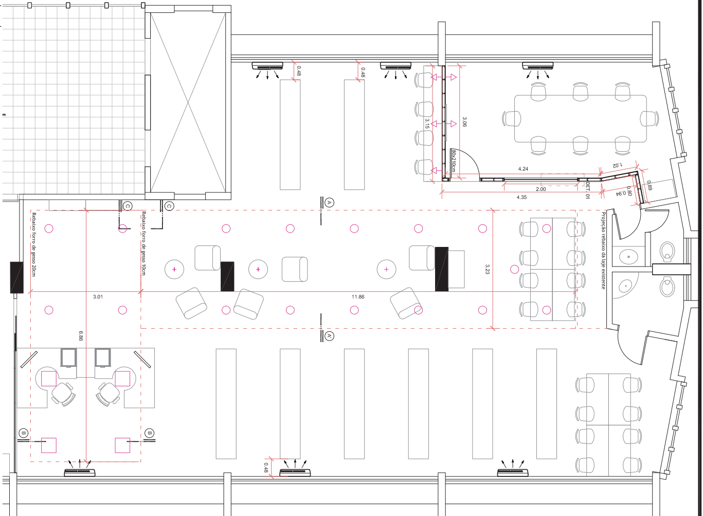
1 Layout 1:75
