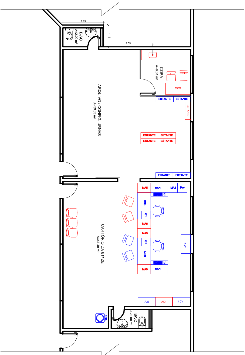
1 LAY OUT ESCALA 1:100
